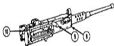
Caliber 50 Machine Gun, Browning, M2, Heavy Barrel, Flexible
